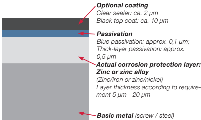
General structure of a galvanic coating
