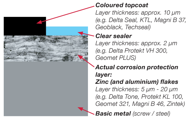
General structure of a zinc flake coating
